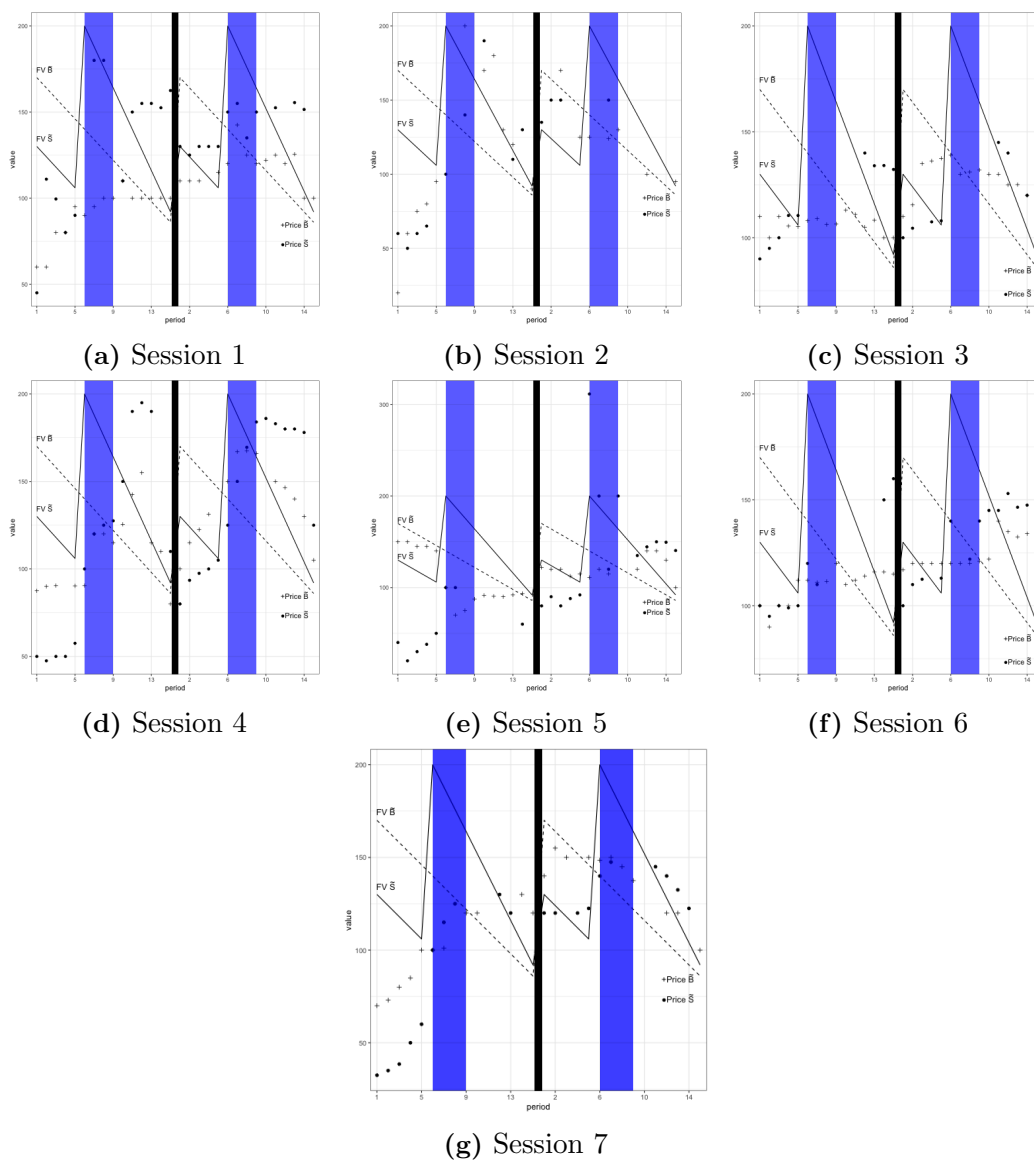
Figure 7: Asset prices and fundamental values per period (2 markets).
